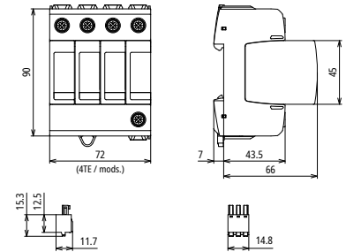
Dimension drawing
