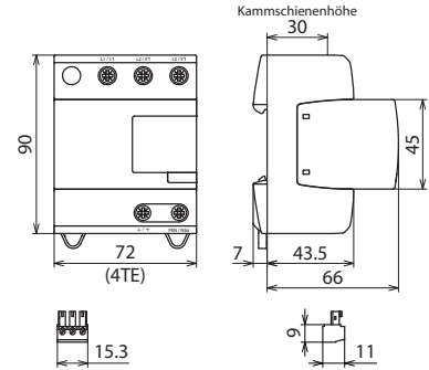
Dimension drawing
