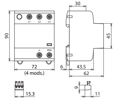
Dimension drawing
